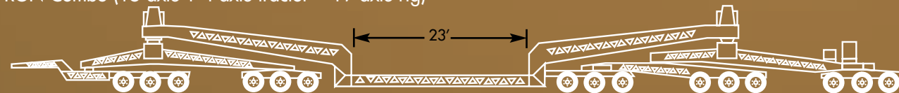
RGN Combo (15 axle + 4 axle tractor = 19 axle rig)
